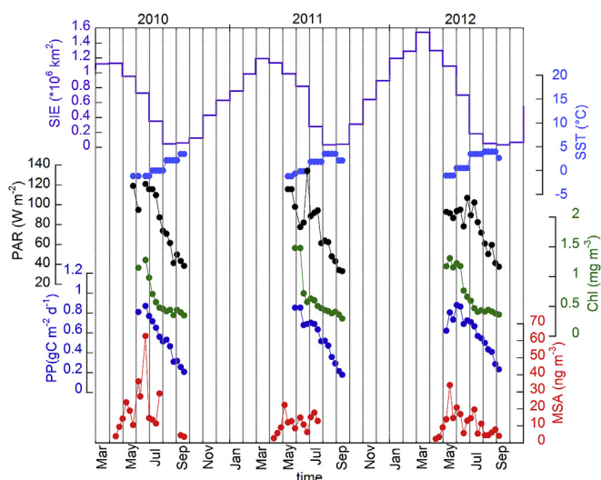
Fig. 8. Three-year evolution of sea ice coverage area (SIE, monthly average), sea surface temperature (SST), photosynthetic active radiation (PAR), Chlorophyll a (Chl- a ), primary production (PP) calculated for the Baffin Bay, and MSA at Thule. SST, PAR, Chl- a and PP and MSA are calculated as 8-day averages.
